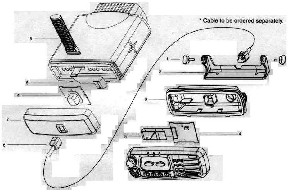
Figure 1 Remote Front and Back Housings
