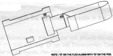
Figure 2 Remote Back Housing PCB with Flex
