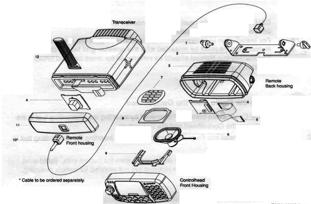
Figure 1 Remote Front and Back Housings
